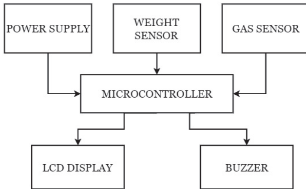
Fig. 1. Block diagram.
