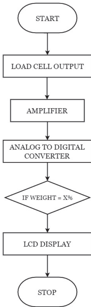
Fig. 3. Flowchart of LPG monitoring.
